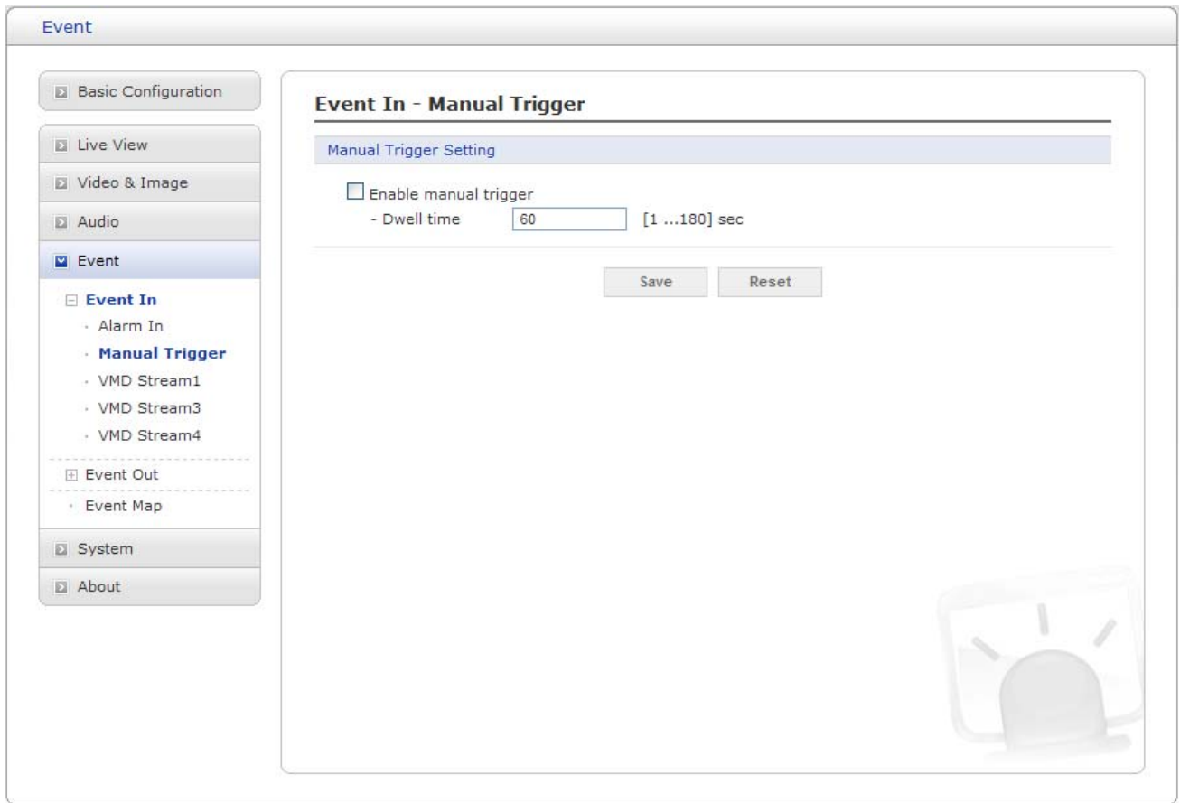
Figure 29. Event / Event In – Manual Trigger
