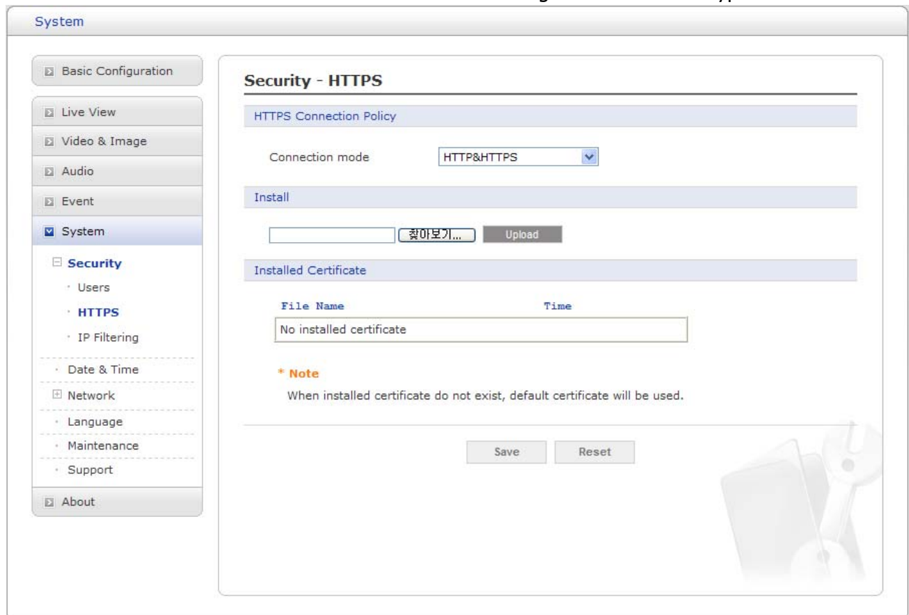
Figure 47. System / Security – HTTPS
