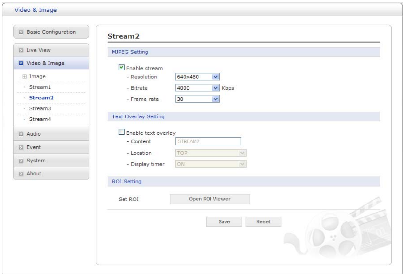
Figure 20. Video & Image / Stream2
