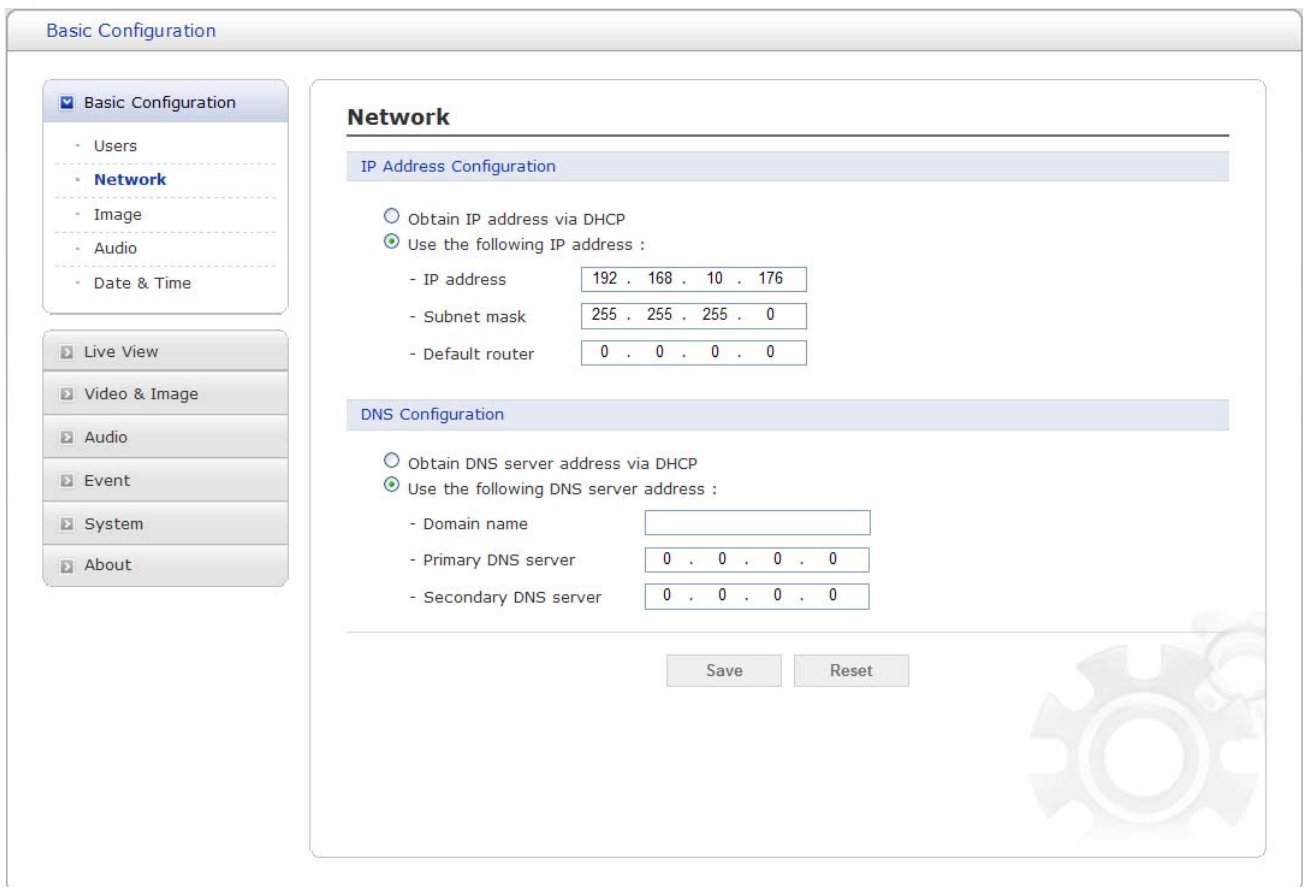
Figure 11. Basic Configuration / Network
