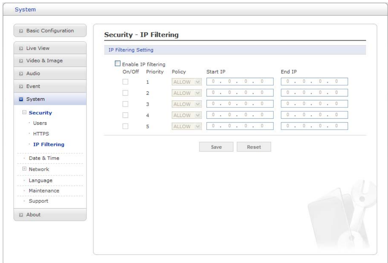
Figure 48. System / Security – IP Filtering
