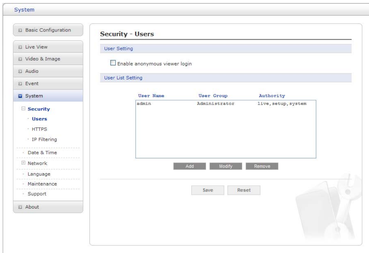
Figure 44. System / Security – Users
