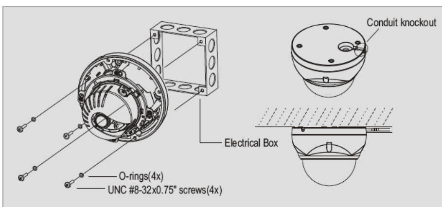
Figure 3. Mount electric box
