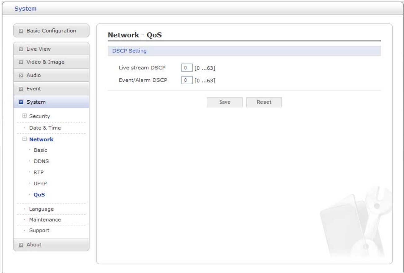
Figure 54. System / Network – QoS
