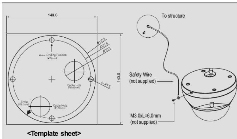
Figure 1. Mounting Hole
