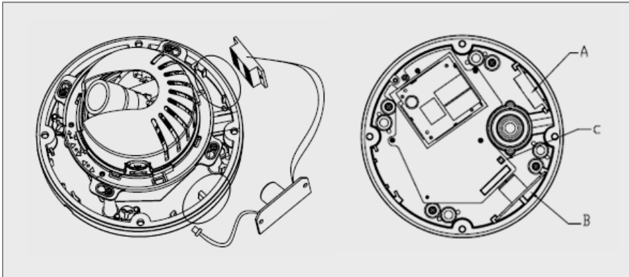
Figure 4. Heater Kit Installation
