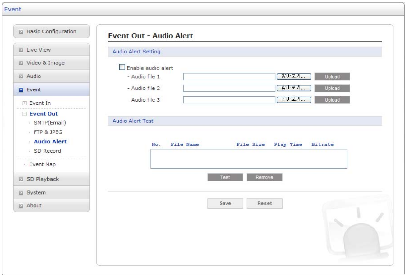
Figure 35. Event / Event Out – Audio Alert.
