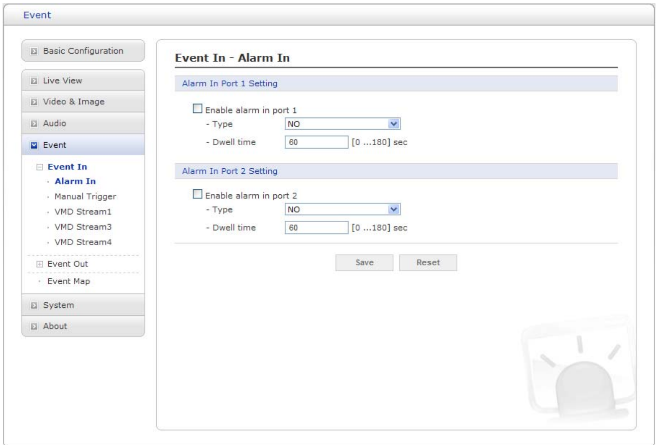
Figure 28. Event / Event In – Alarm In
