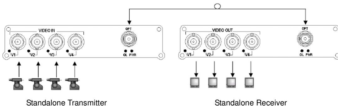
Fig 4.1 Standalone unit to Standalone unit connection diagram
