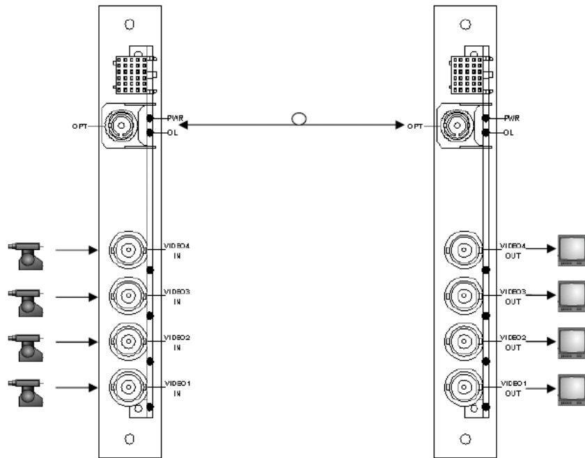
Card Module Transmitter
