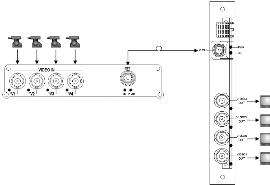
Standalone Transmitter
