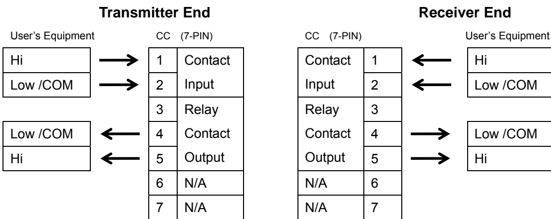
Fig. 4.4.2 Connector Pin Assignments for Contact Closure/TTL input and Normally Open (NO) output at CC port
