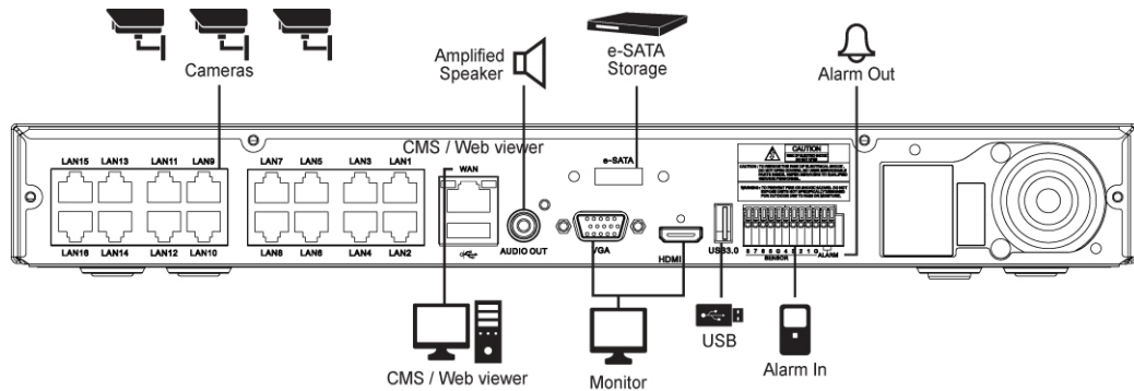
Figure 2-1 Connection map
